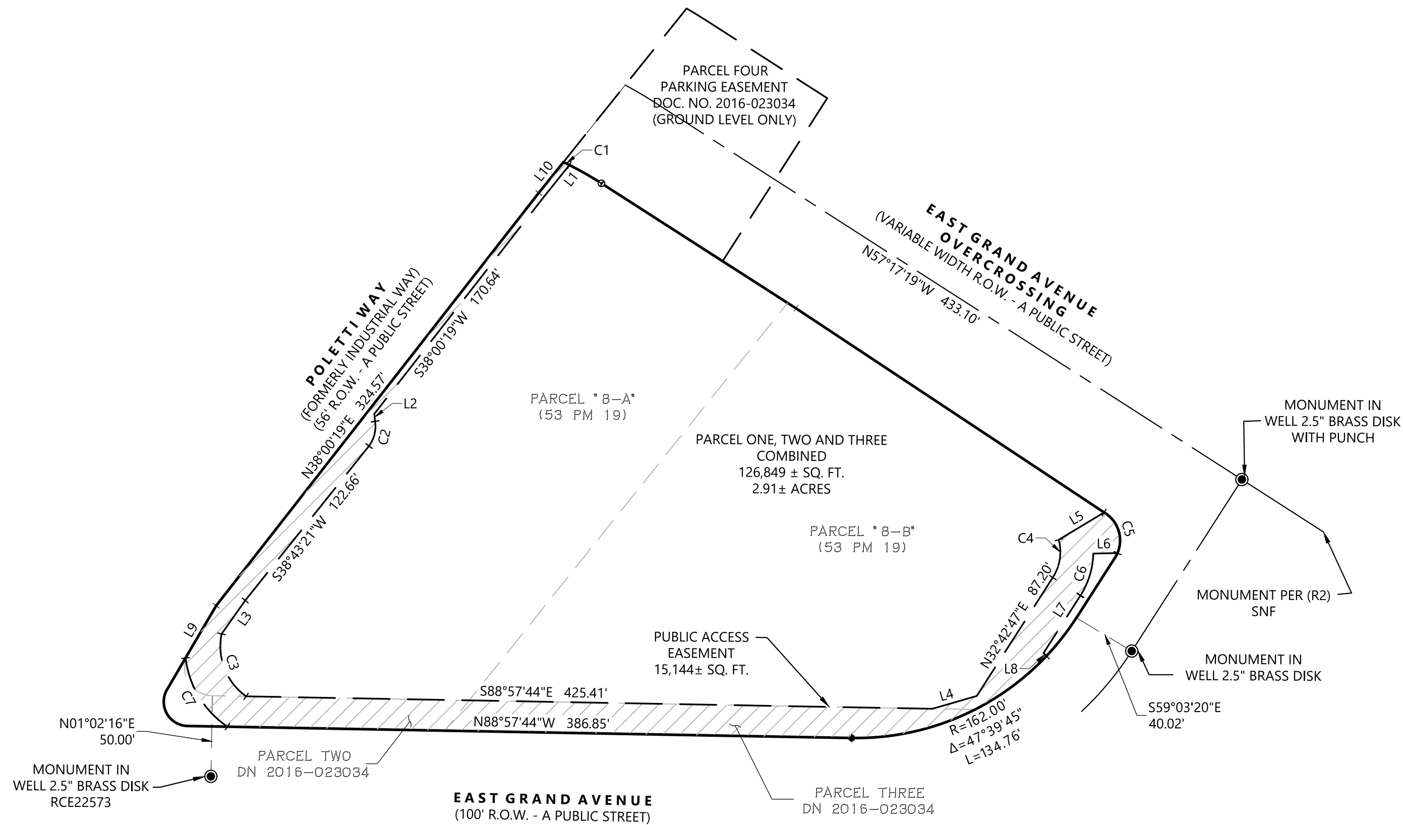
DETAIL "A" 1" = 60'
