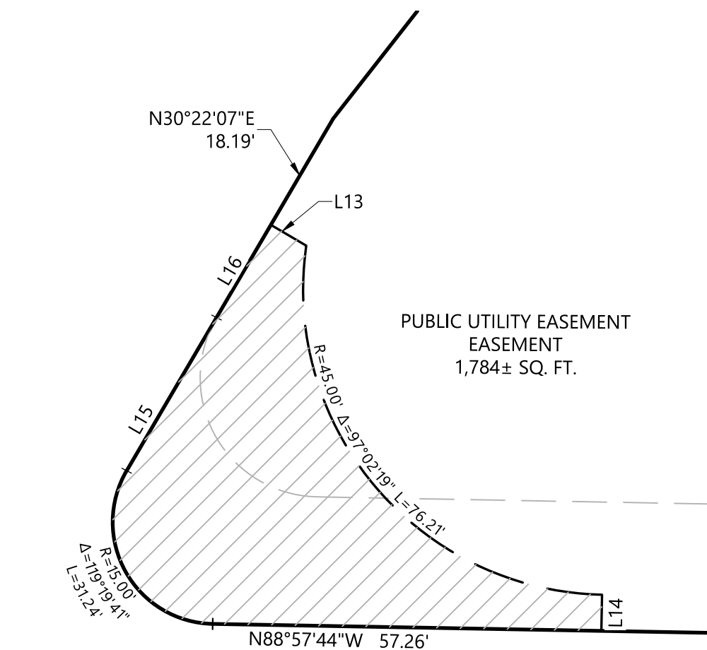
DETAIL "C" 1" = 20'
