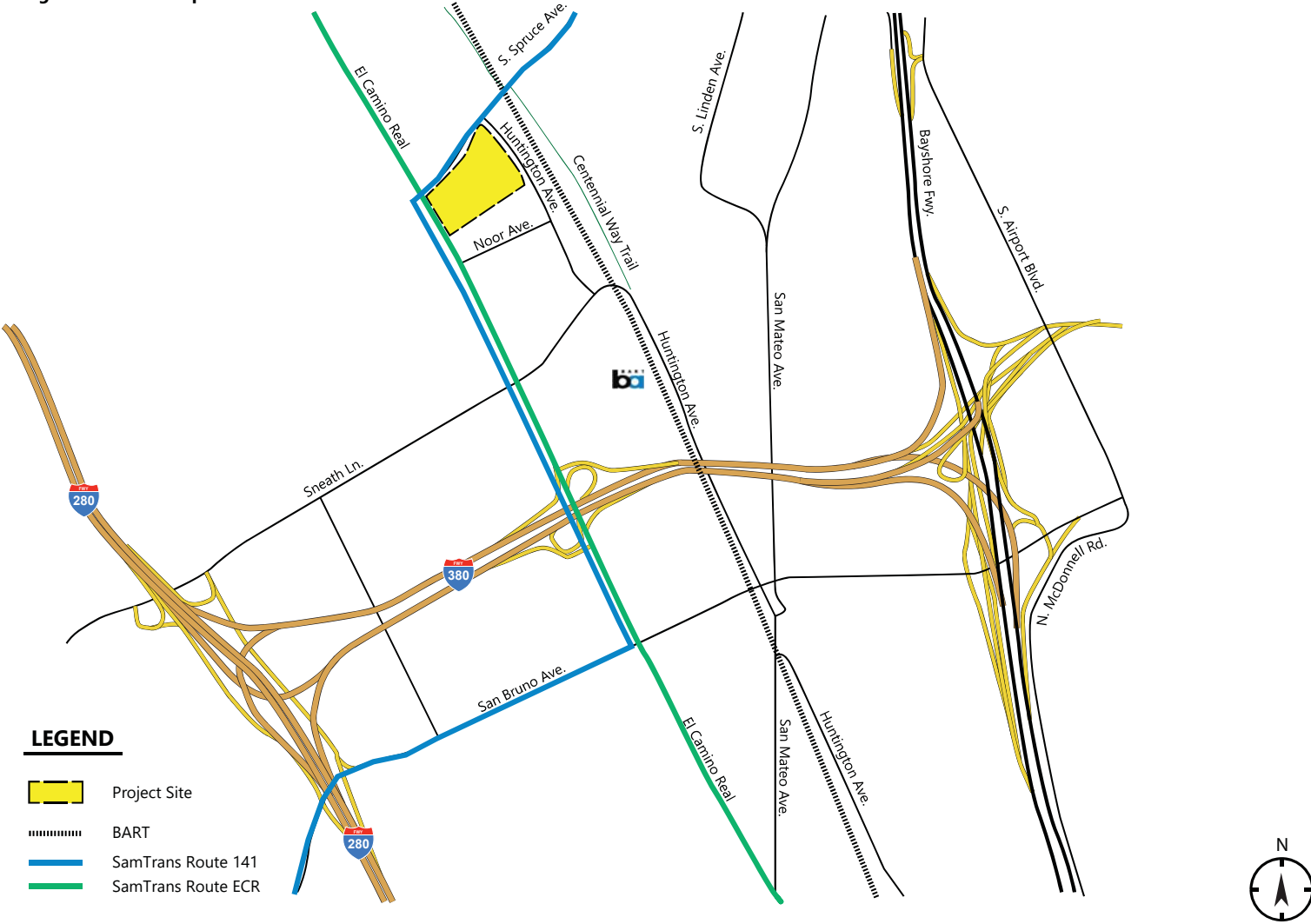
Figure 3: Transit Map
