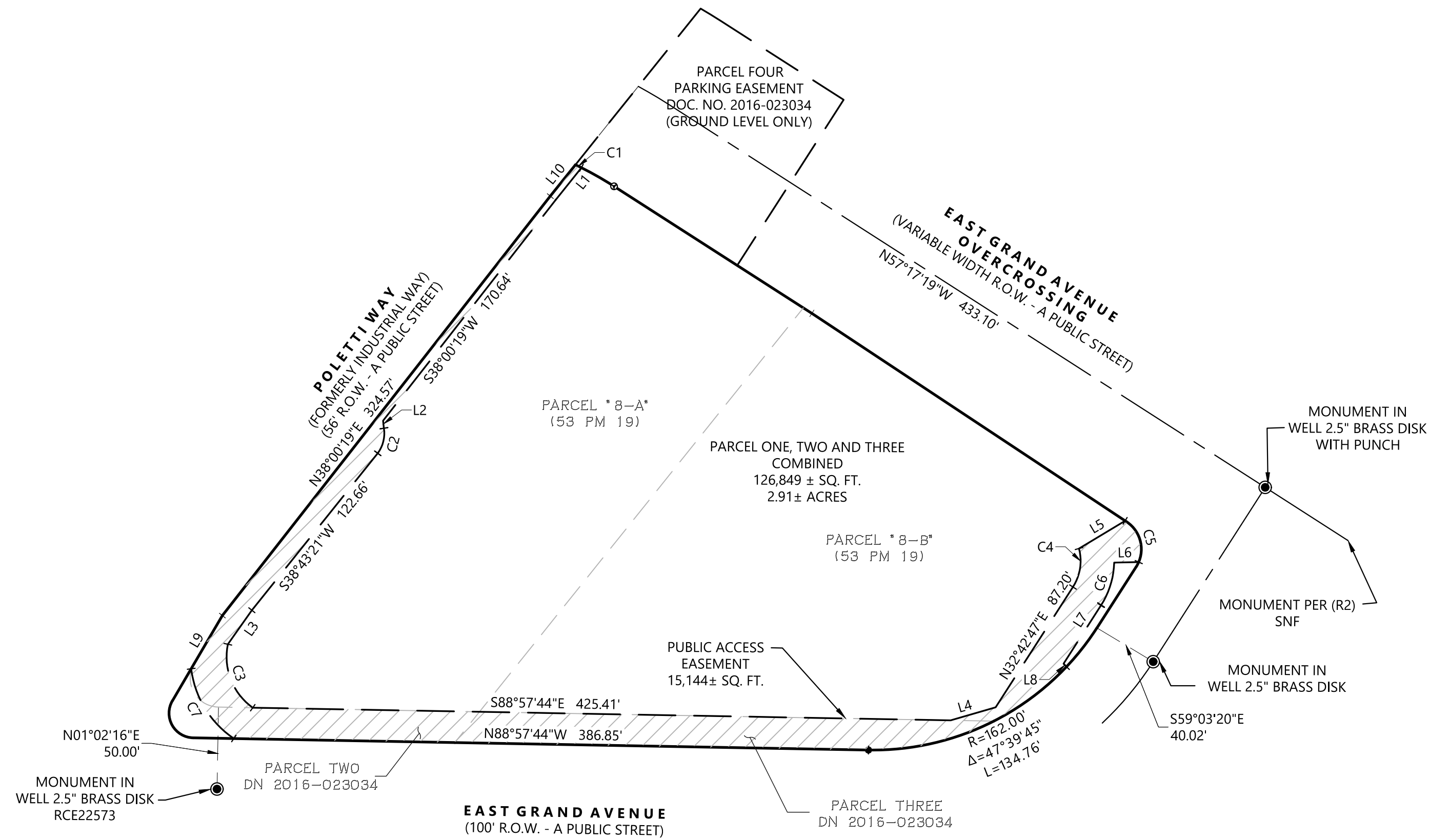
DETAIL "A" 1" = 60'
