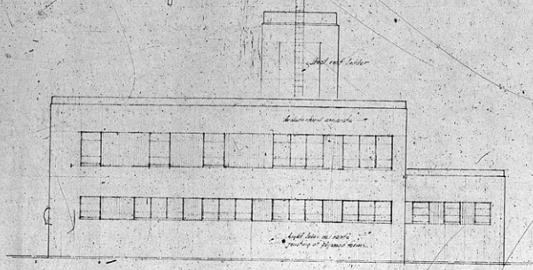
WEST ELEVATION
