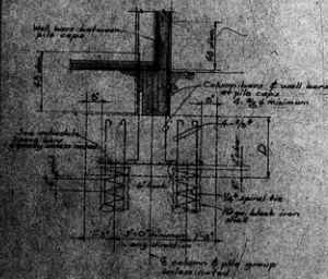
TYPICAL PILE CAP
