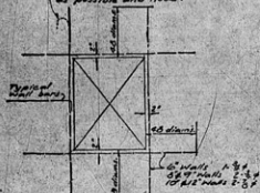
MINIMUM STEEL AROUND OPENING IN WALL
