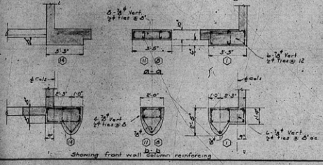
Showing front wall column reinforcing
