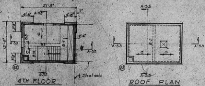
ROOF PLAN
