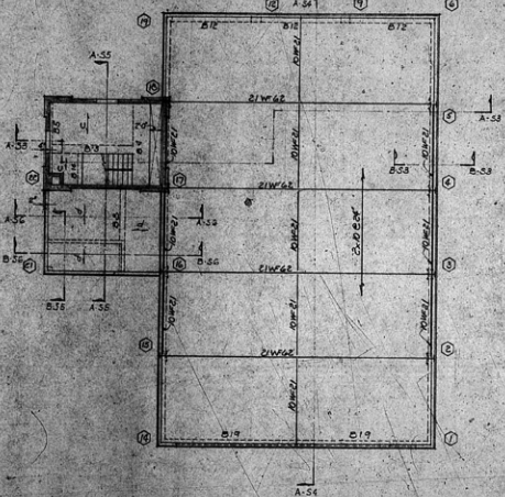
3RD FLOOR ROOF FRAMING PLAN
