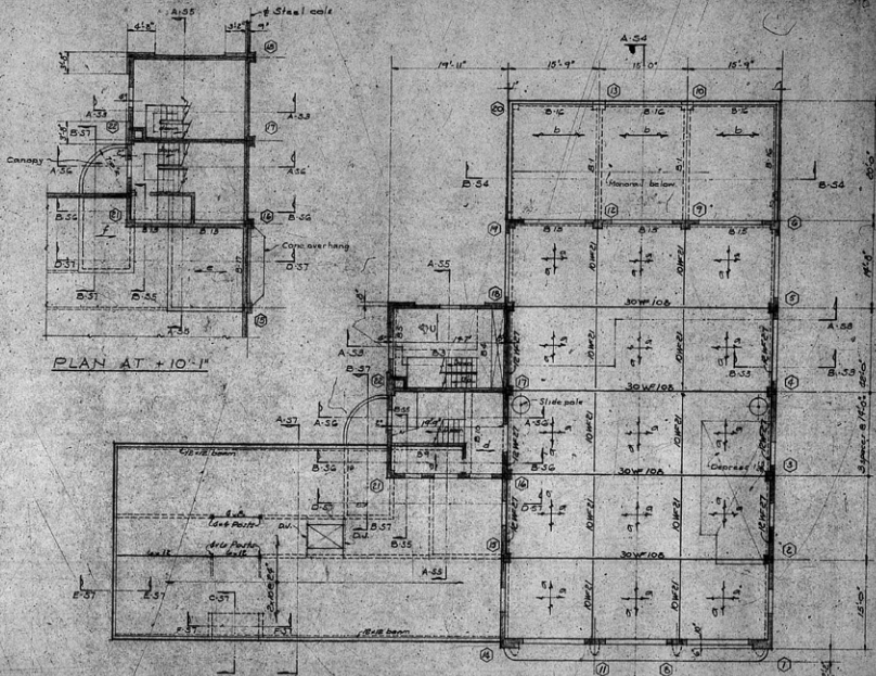
ROOF & 2ND FLOOR FRAMING PLAN
