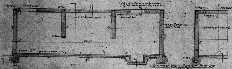
SECTION THRU ENGINE TEST PIT
