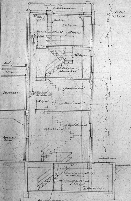
SECTION 15 THROUGH TOWER Scale 1/8" = 1'-0"
