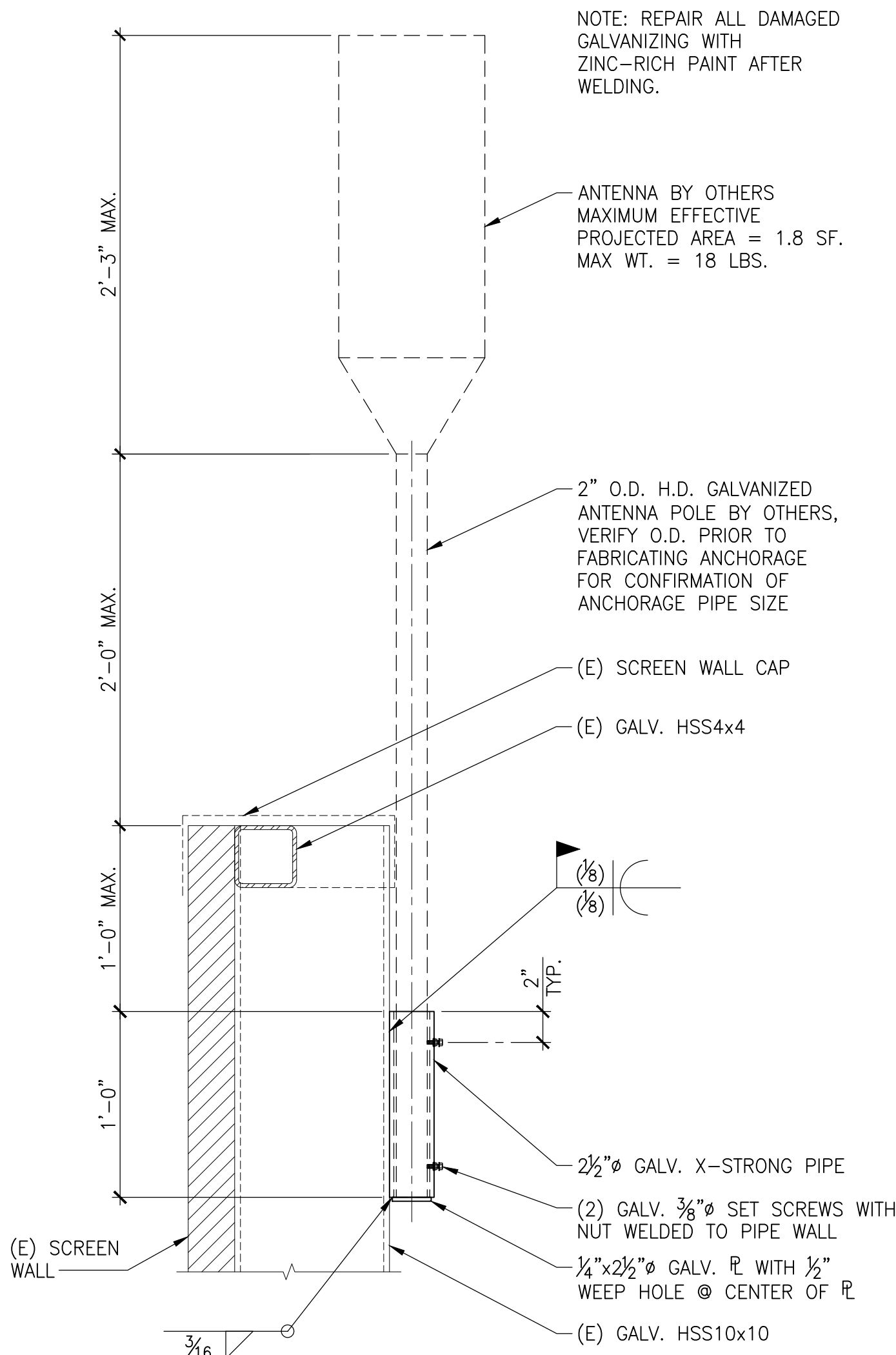
6 ANTENNA POLE ANCHORAGE DETAIL AT TOP OF SCREEN WALL SCALE: 1 1/2"=1'-0"
