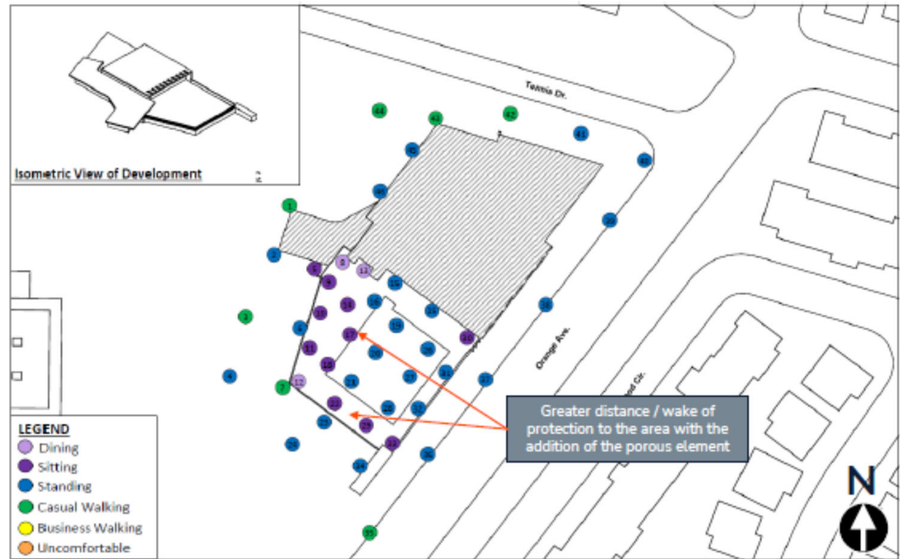
Pedestrian Wind Comfort Conditions - Operating Hours (January to December, 6:00am - 9:00pm)
