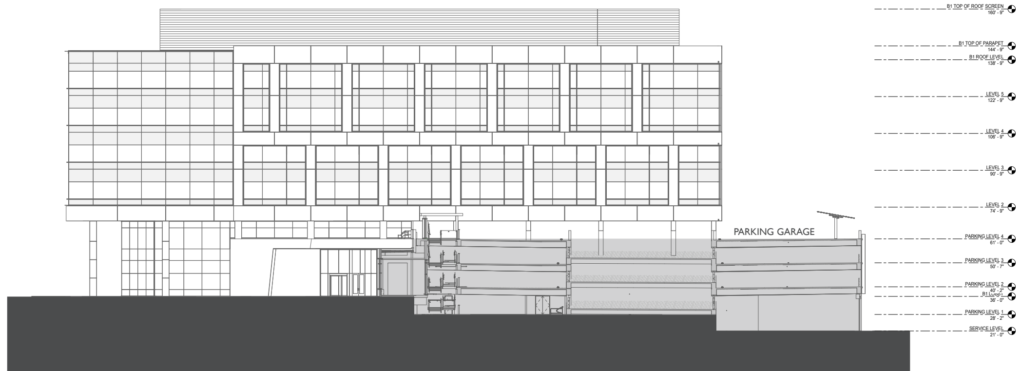
2 WEST ELEVATION
