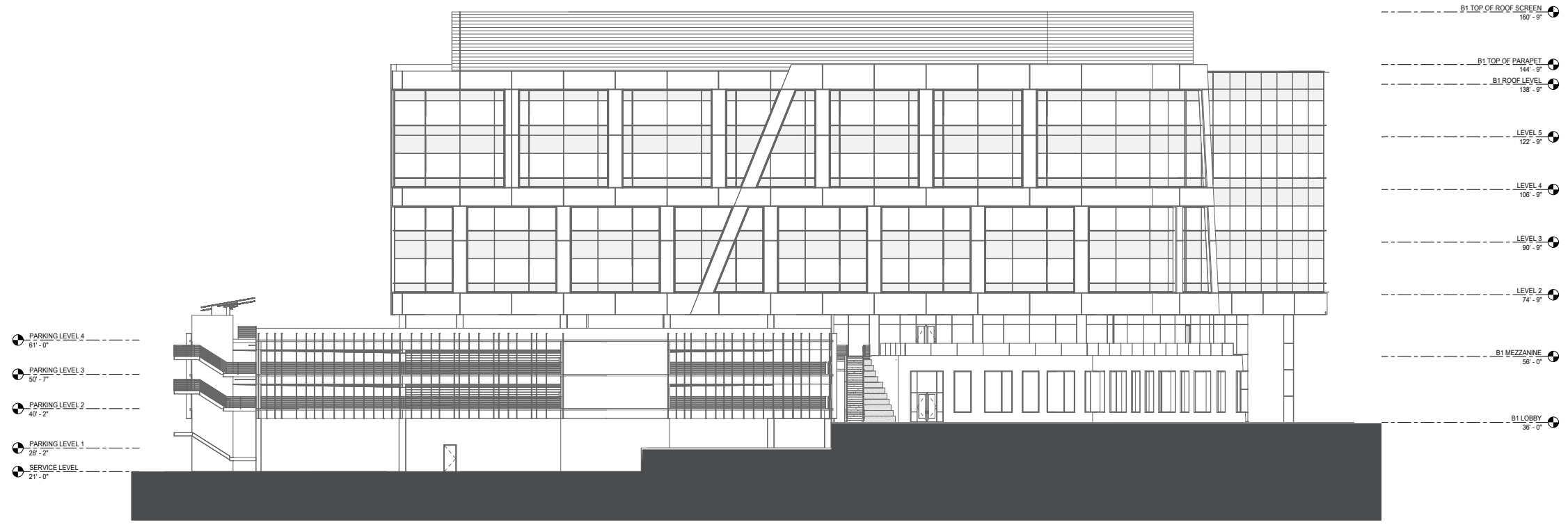
1 EAST ELEVATION
